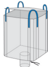
Open top with flap discharge spout.
